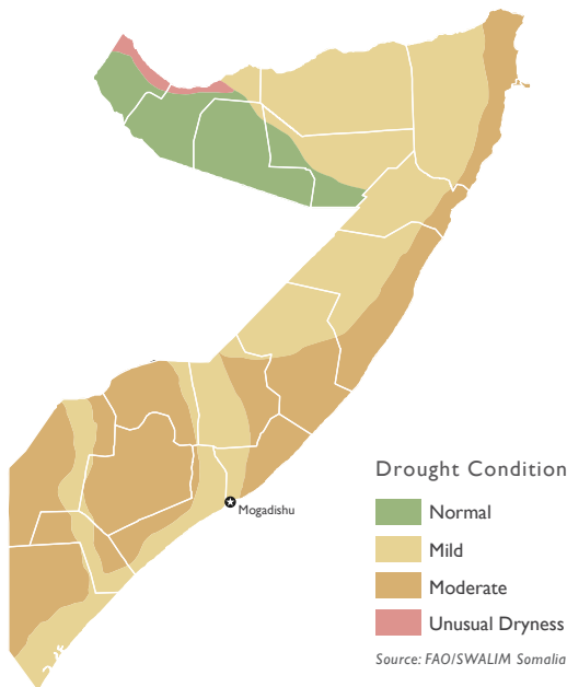
Drought Severity Map, August 2021
