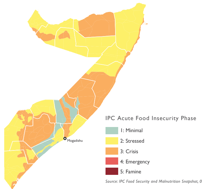
Projected Acute Food Insecurity, October Through December 2021
