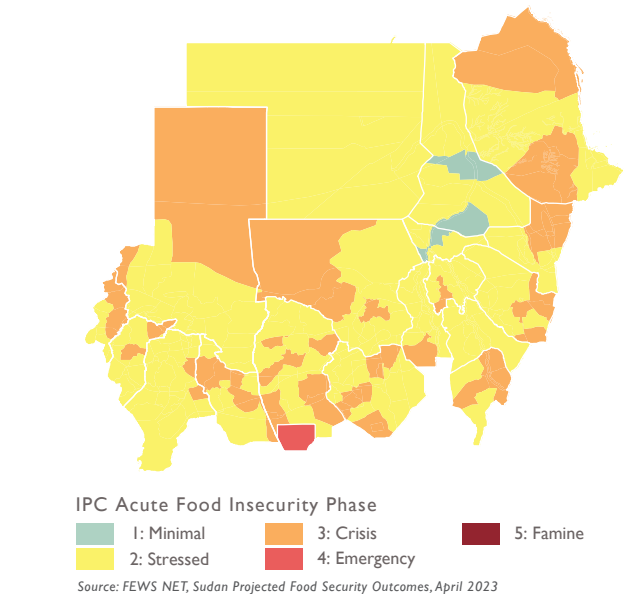
Projected Food Security Outcomes, April–May 2023
